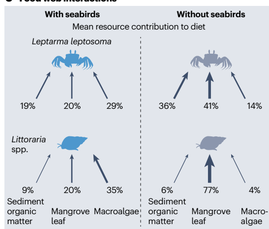
Fig. 3 | Seabird impacts on adjacent marine ecosystems. a, Impacts on temperate (left) and tropical (right) ecosystems. b, Coral and reef fish growth rates are boosted by seabird nutrients. c, Seabird presence reshapes food web
