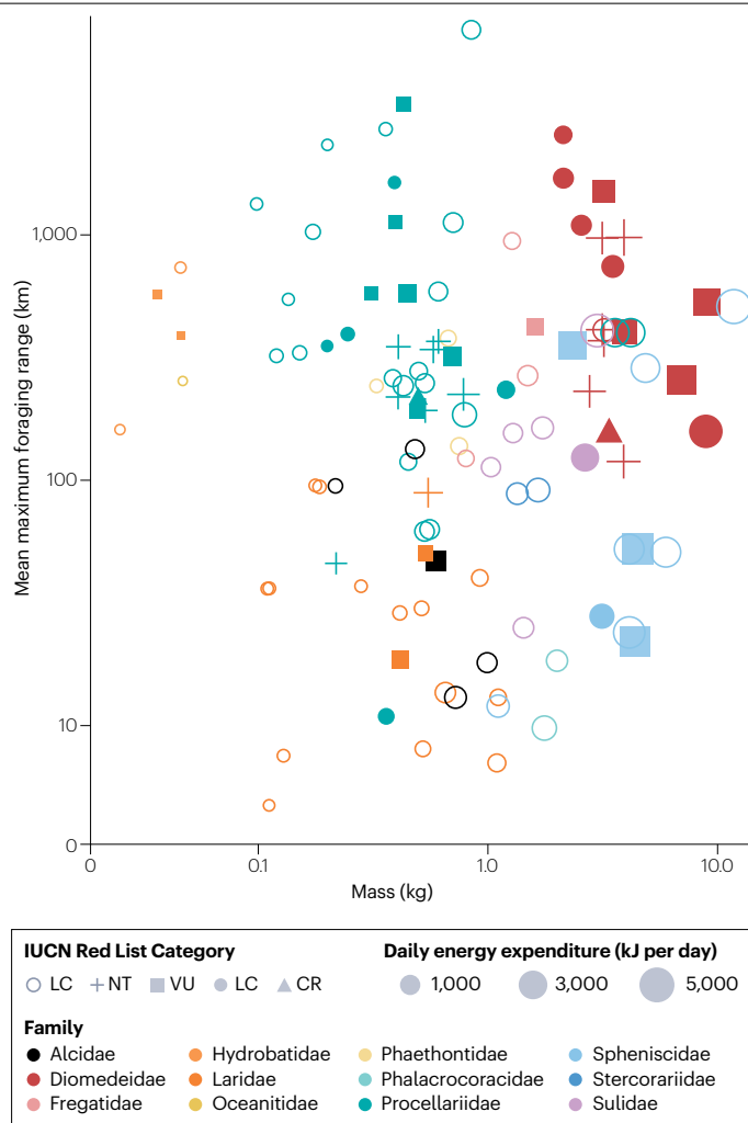
Fig. 2 | Seabird mass and foraging range. The relationship between mean bird mass (kg) and foraging range for breeding adult seabird species (km). Species are categorized by International Union for Conservation of Nature (IUCN) Red List conservation status (symbols), daily energy expenditure (kJ per day; point size) and taxonomic family (colour). Data on mean bird mass are from ref. 180. Data on mean seabird foraging ranges were collated for breeding adult seabirds where data exist within ref. 181 via Google Scholar searches ( n = 110 seabird species). Where means were not available, medians were used. Daily energy expenditure was calculated via the Seabird FMR Calculator in ref. 16. See Supplementary information for further information and complete data sources. IUCN Red List categories: least concern (LC), near threatened (NT), vulnerable (VU), endangered (EN) and critically endangered (CR).
