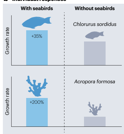
Fig. 3 | Seabird impacts on adjacent marine ecosystems. a, Impacts on temperate (left) and tropical (right) ecosystems. b, Coral and reef fish growth rates are boosted by seabird nutrients. c, Seabird presence reshapes food web
