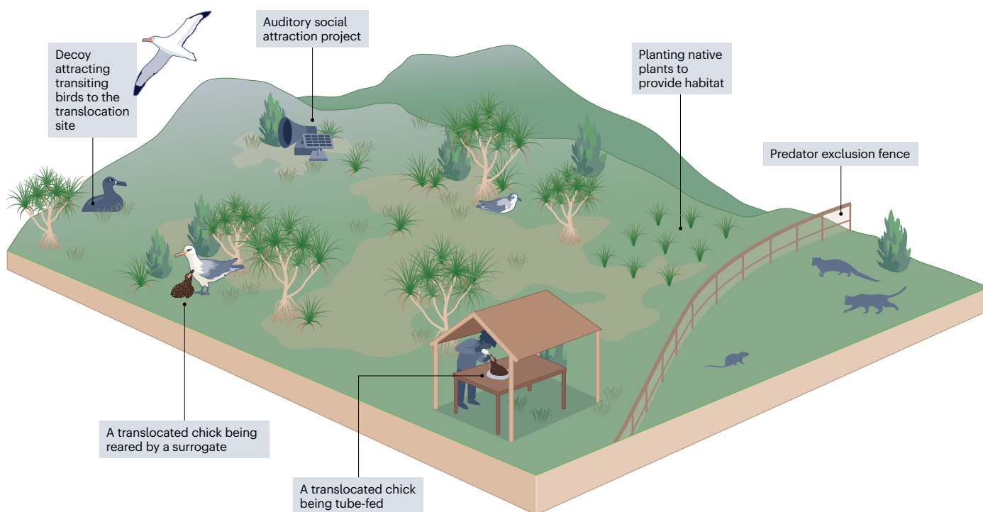
Fig. 4 | Seabird restoration methods. Predator exclusion fencing prevents invasive mammalian predators from accessing the newly established seabird colonies. Plantings of native plant species can provide habitat for seabirds to roost. Use of decoys can attract seabirds to suitable translocation sites. Auditory
